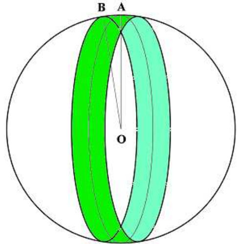
FIG. 1: The visibility band (shaded) of a set of spherical-crystal lattice planes whose trace follows the great circle through A. Lattice fringes disappear as the electron beam is tilted from any point along the trace in a direction perpendicular to the trace circle by an angle greater than angle AOB = \alpha_{max} , the visibility band halfwidth.
