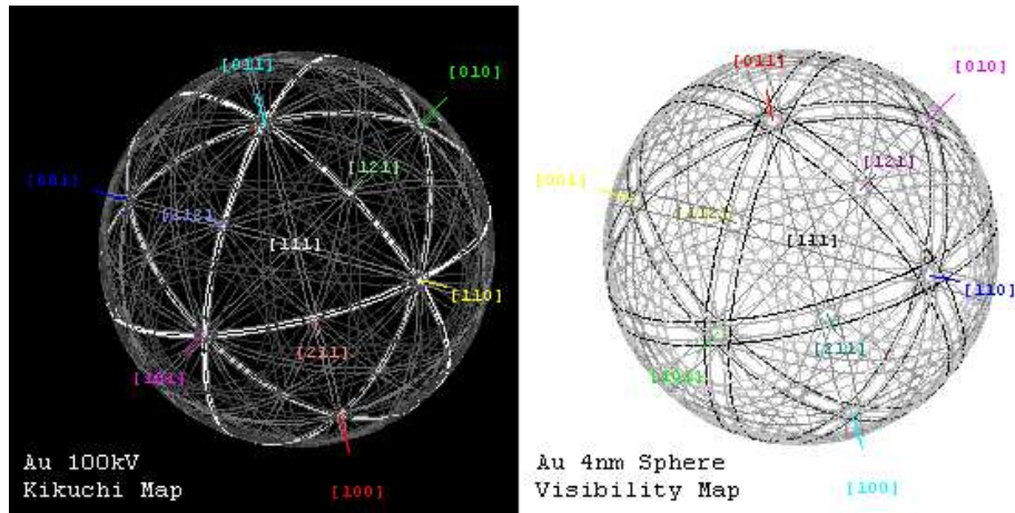
FIG. 3: Comparison of Kikuchi map (left) to a fringe-visibility maps (right) for a t = 4 [nm] single-crystal gold sphere imaged at 100[kV]. To first order, band-widths in the former (where t \gg t_{crit} ) are proportional to \lambda/d , while band-widths in the latter (where t \ll t_{crit} ) are proportional to d/t . Band boldness and d-spacing are correlated.
