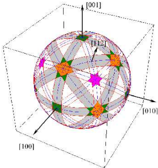
FIG. 2: One fringe-visibility map for a spherical fcc crystal.
