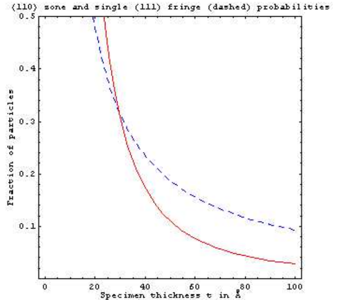
FIG. 7: The cross-over in abundance of cross-fringe versus single-fringe particles, with decreasing size.
