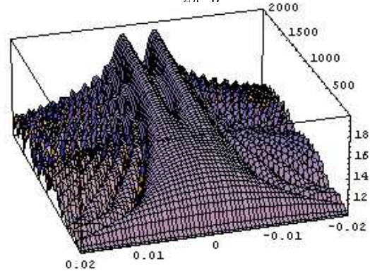
FIG. 15: Logarithmic fringe-intensity profile ( d = 2\text{\AA} and \lambda = 0.01\text{\AA} ) for a spherical particle whose diameter t is given in Angstroms by the top-labeled axis (running front to back), as a function of “tilt from edge-on in radians” on the bottom-labeled axis (running left to right).
