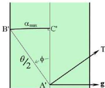
FIG. 14: A segment of a continuous visibility band, with half of the visibility “tilt range” marked by segment A'B'.
