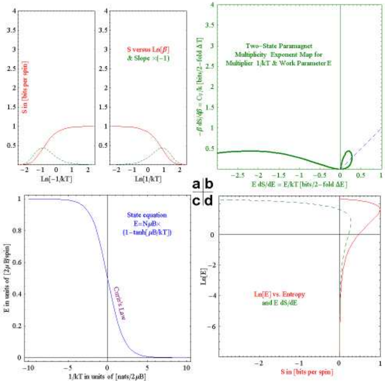
FIG. 4: Plots of the dependence of entropy on energy per spin for a two-state paramagnet consisting of 10 non-interacting spins. (a) S/N and its slope \frac{C_V}{Nk} (dashed line) vs \ln(\frac{1}{kT}) , (b) multiplicity exponent map \frac{C_V}{Nk} vs \frac{E}{NkT} , (c) equation of state plot E/N vs dE/dS = \frac{1}{kT} , and (d) \ln(E/N) vs \frac{S}{N} and its slope \frac{E}{NkT} (dashed line). The layout is similar to that in Figs. 2 and 3 except that 1/kT replaces kT on the left hand side. As discussed in the text, 1/kT runs from \infty to -\infty as T goes from 0^+ to 0^- , the upper left and lower right entropy plots show a single maximum, and in the exponent map, the heat capacity remains positive while E/kT takes on negative values that correspond to the negative reciprocal temperature side of the entropy peak. If the energy zero is reset halfway between minimum and maximum energy values, the lower right entropy peak becomes symmetric, and the loop in the positive quadrant of the exponent map disappears.
