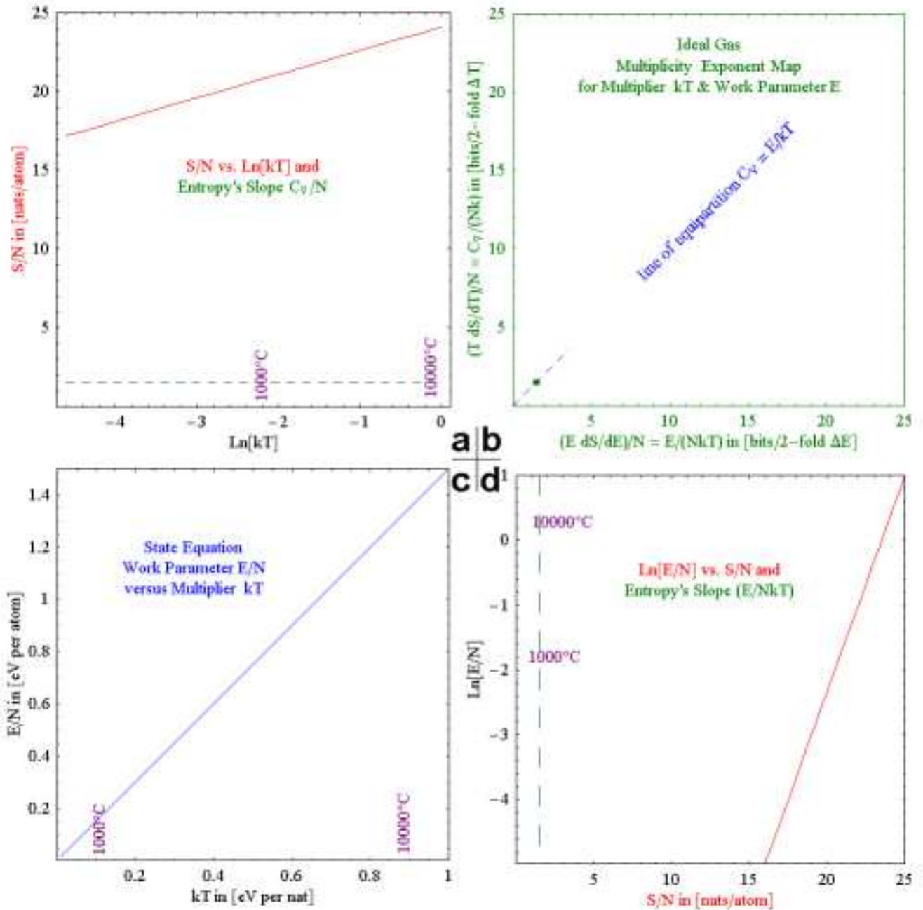
FIG. 2: Plots of the dependence of the entropy on the energy E and energy multiplier kT , for the ideal (Sakur-Tetrode) 10-atom argon gas of Fig. 1 in a fixed volume of 0.4 zeptoliters. (a) S and its slope \frac{C_V}{k} (dashed line) vs \ln(kT) , (b) multiplicity exponent map \frac{C_V}{k} vs \frac{E}{kT} , (c) equation of state plot E/N vs dE/dS = kT , and (d) \ln(E/N) vs \frac{S}{N} and its slope \frac{E}{kT} (dashed line). Note how the lower left corner panel axes lead into both adjacent panels, and how the derivative plots in turn lead to the exponent map in the upper right, which for the case of this simple quadratic system yields a single point at \frac{C_V}{N} = \frac{E}{NkT} = \frac{3}{2} on the “line of equipartition.”
