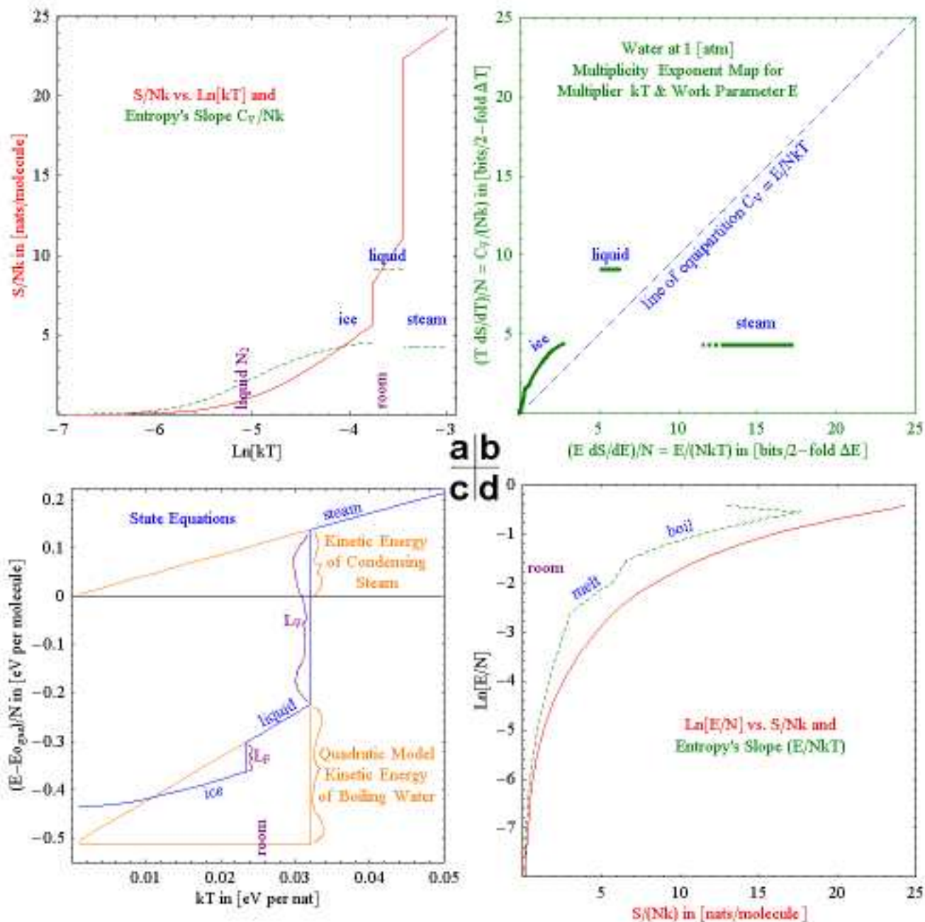
FIG. 3: Plots of the dependence of entropy on energy per molecule for a steam, water, and Debye model ice system ( \theta = 333 K assuming a sound speed near 3500 m/s). For simplicity, we have ignored the effect of volume changes on energy, and thus for example, steam has a lower heat capacity than it would in an experiment done at 1 atm. (a) S/N and its slope C_V/Nk (dashed line) vs \ln(kT) , (b) multiplicity exponent map \frac{C_V}{Nk} vs \frac{E}{NkT} , (c) equation of state plot E/N vs dE/dS = kT , and (d) \ln(E/N) vs \frac{S}{N} and its slope \frac{E}{NkT} (dashed line). The layout of the panels is similar to that in Fig. 2, but curve shapes are now complicated by two phase changes, and the Debye model “freezing out” of thermal energy storage modes in the model used for ice. As discussed in the text, locally defined energy zeros are useful in understanding features seen in the lower left panel, phase changes are more clearly distinguishable in the upper left than in the lower right entropy plots, and the plots on the right side vary drastically with the choice of the energy zero.
