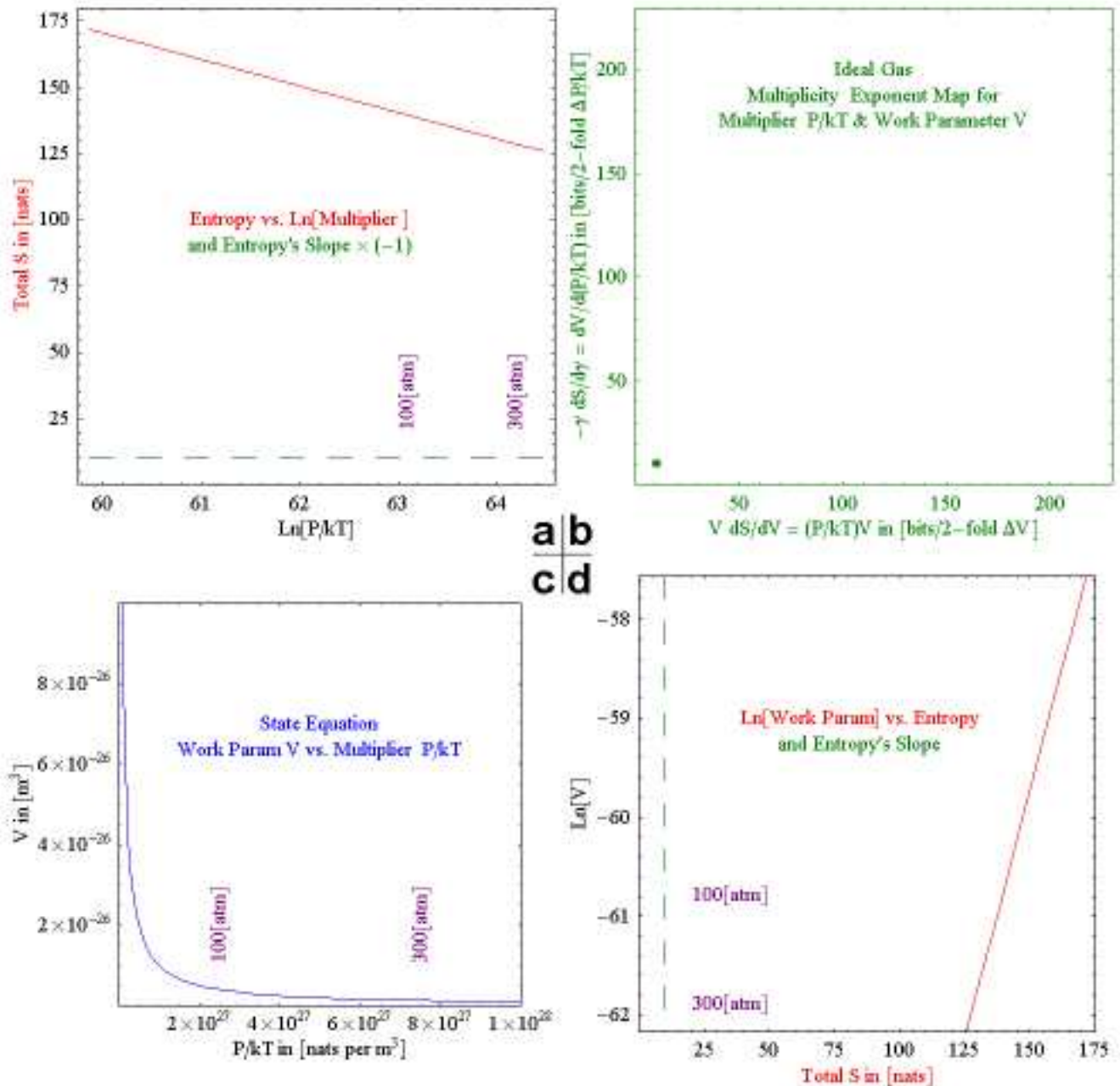
FIG. 1: Plots of the dependence of the entropy on the volume, and the latter's Lagrange multiplier \gamma = P/kT , for an ideal (Sakur-Tetrode) 10-atom argon gas at 290 K. (a) S (solid line) and its slope \gamma dS/d\gamma (dashed line) vs \ln \gamma , (b) the multiplicity exponent map \gamma dS/d\gamma vs V dS/dV , (c) state equation plot of V vs dS/dV = \gamma = P/kT , (d) \ln V vs S and its slope V \frac{dS}{dV} (dashed line). The entropy expression used for this is \frac{S}{k} = N(\ln[\frac{V}{N}] + (\frac{3}{2}) \ln[\frac{4\pi m E}{3N h^2}] + \frac{5}{2}) , where V is total volume, E is total energy, N is number of atoms, m is atomic mass, and h is Planck's constant. Note that Boyle's Law appears in the ideal gas equation of state plot in the lower left, that the adjacent plots show the entropy to be a monotonic increasing function of both V and P/kT , and that the exponent map on the upper right shows the log-log derivative of the multiplicity for both V and P/kT to be fixed at the number of particles N = 10 .
