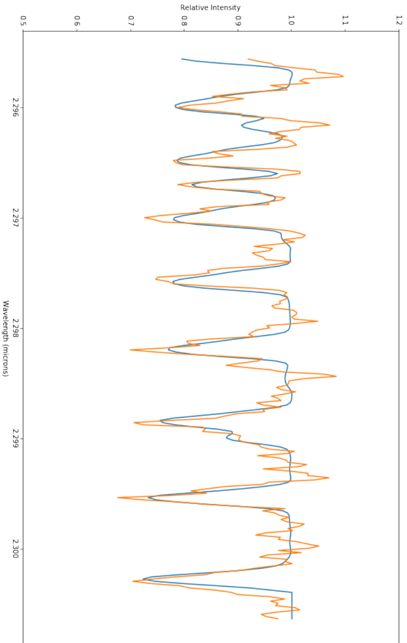
Figure 46 Synthetic overlay (blue) on top of the data (orange) for the four fit parameters returned by emcee to best match the CSHELL spectrum of radial velocity standard HD 122120 corresponding to T = 3940 \pm 20 K, v \sin i = 8.8 \pm 0.1 km s -1 , r_k = 0.00 \pm 0.01 , and dx = -12.72 \pm 0.02 .
