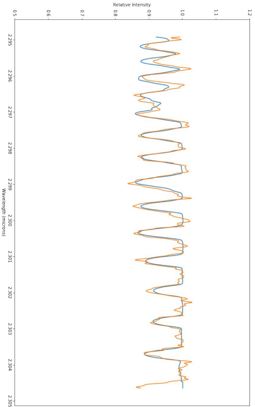
Figure 54 Synthetic overlay (blue) on top of the data (orange) for the four fit parameters returned by emcee to best match the CRRES spectrum of object GY 23 corresponding to T = 4120 \pm 20 K, v_{\text{ sini}} = 20.9 \pm 0.2 km s -1 , r_k = 0.52 \pm 0.01 , and dx = -18.98 \pm 0.06 .
