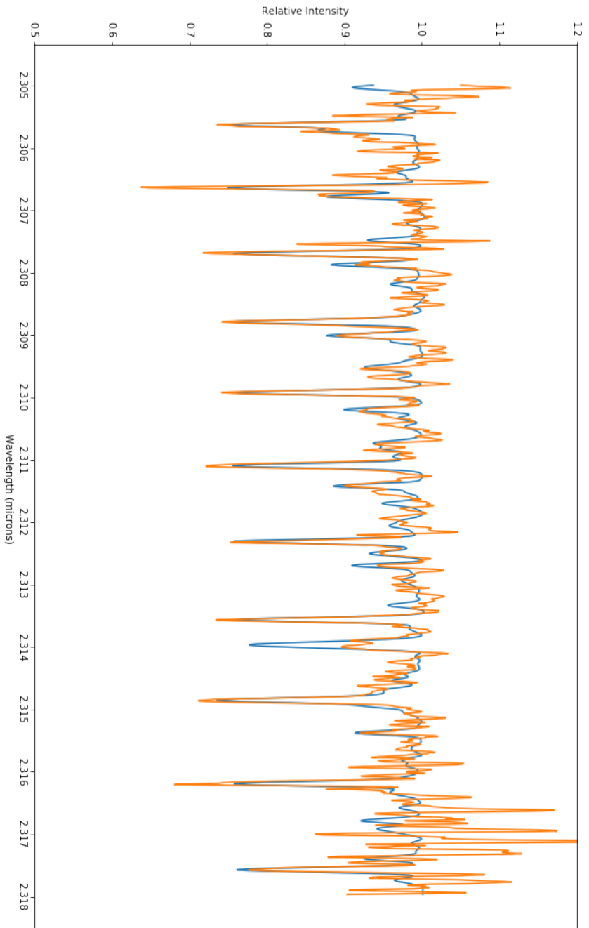
Figure 78 Synthetic overlay (blue) on top of the data (orange) for the four fit parameters returned by emcee to best match the iSHELL spectrum of order 224 of object GY 284 corresponding to T = 3500 \pm 20 K, v_{\text{simi}} = 5.90 \pm 0.14 km s ^{-1} , r_k = 35 \pm 0.01 , and dx = -16.20 \pm 0.02 .
