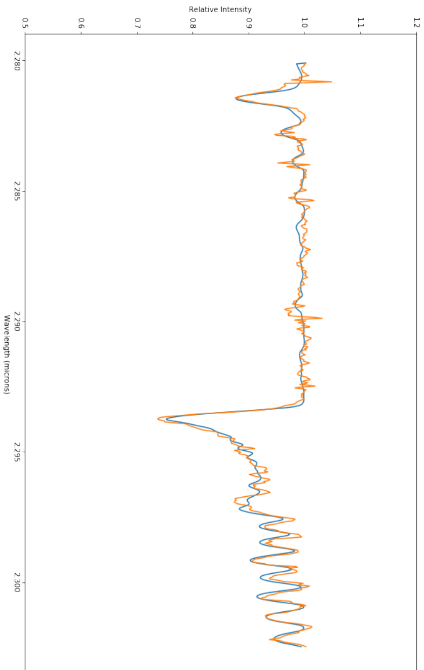
Figure 6 Synthetic overlay (blue) on top of the data (orange) for the four fit parameters returned by emcee to best match the NIRSPEC spectrum of object GSS 29 corresponding to T = 4360 \pm 40 K, v \sin i = 36.6 \pm 0.4 km s -1 , r_k = 0.3 \pm 0.02 , and dx = 0.84 \pm 0.08 .
