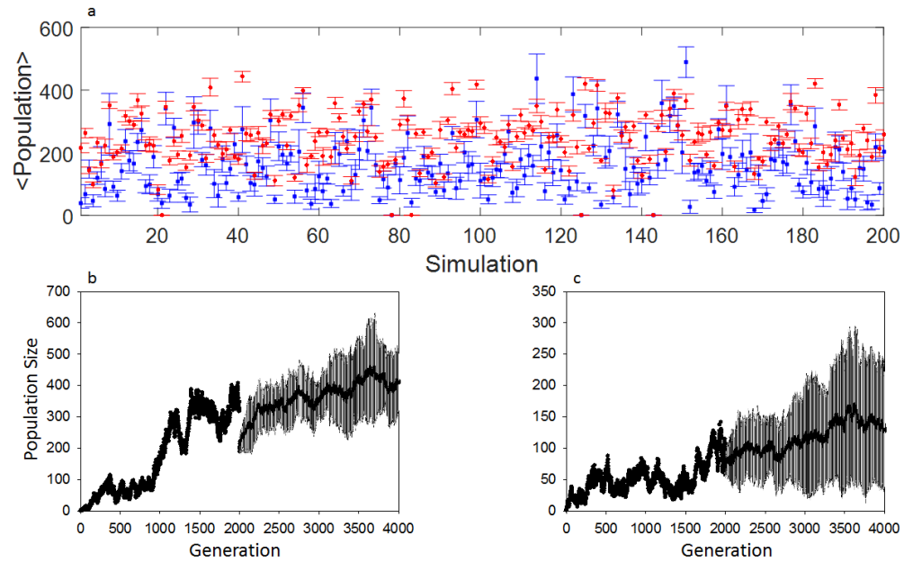
Figure 4.10. Ten Trials at \delta_c = 0.28 with 50% Mass Death: Asexual Fission — Panel a represents average population size of the last 500 generations pre- (blue circles) and post- (red circles) extinction. Panels b and c represent chosen simulations 126 and 116, respectively. Error bars show the standard deviation in population size over ten mass extinction simulations.
