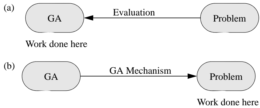
Figure 1. A GA with (a) traditional and (b) task-specific operators.
