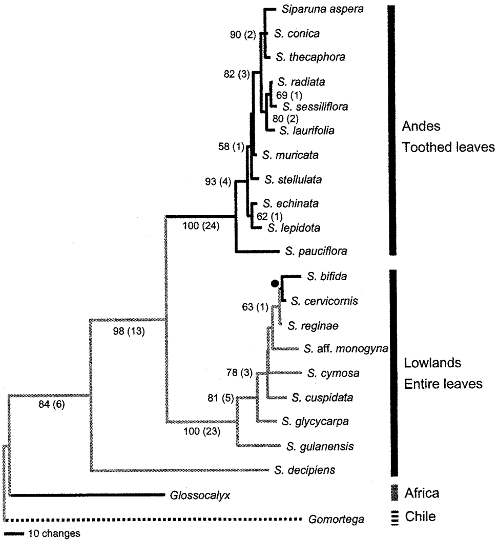
FIGURE 1. One of six equally parsimonious trees resulting from analysis of ITS and trnL-trnF sequences of Siparunaceae ( L = 658, CI = 0.69, RI = 0.85 ). Branch lengths are proportional to numbers of substitutions. Bootstrap support values >50\% shown at nodes are based on 1,000 replications; decay indices follow in parentheses. A node collapsing in the strict consensus is indicated with a solid circle. Dioecious lineages are shown in black, monoecious ones in gray, and perfect-flowered ones dashed. For full species names with authors see Table 1.
