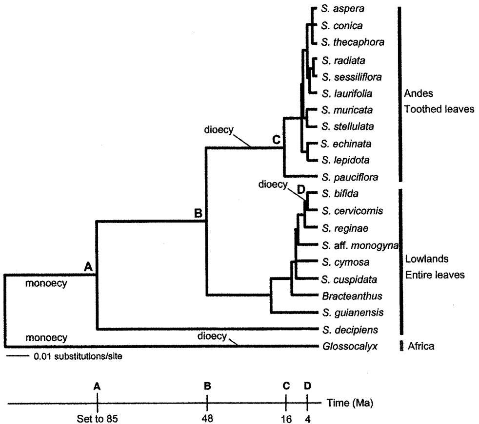
FIGURE 2. Single highest likelihood tree for Siparunaceae found under the GTR + \Gamma + P_{inv} + clock model. The preferred scenario (three gains of dioecy from monoecy) is illustrated here, based on arguments provided in the text; the sister groups of Siparunaceae have bisexual flowers. Based on either the separation of Africa and South America (complete by 90 Ma) or the oldest fossils of the sister clade of Siparunaceae (86–88 Ma), a minimum age for Siparuna (node A) is 85 Ma. Node B denotes the divergence of the Andean clade, node C the onset of major diversification in the Andean clade, and node D the minimum age of S. bifida and S. cervicornis . All nodes may underestimate ages because of extinction. See text for standard deviations on all estimates.
