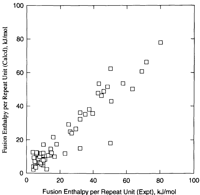
Fig. 2. A comparison of the calculated and experimental fusion enthalpies ( \text{kJ mol}^{-1} ) of 64 polymers.
