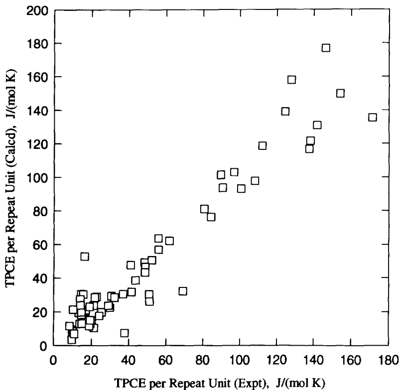
Fig. 1. A comparison of the calculated and experimental fusion entropies ( \text{J mol}^{-1} \text{K}^{-1} ) of 64 polymers.
