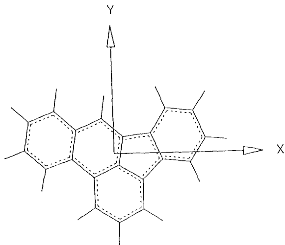
Fig. 1. The moment of inertia ( I ) for benzo[b]fluoranthene is illustrated. The molecular plane coincides with the x, y plane. All PAHs in the training set were aligned based on I . The x and y axes are defined as described in the Methodology under CoMFA alignment and analysis .
