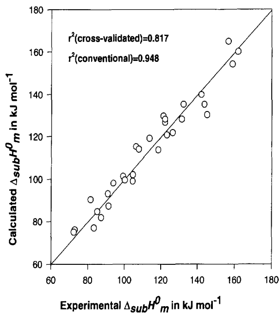
Fig. 2. Calculated versus experimental sublimation enthalpies \Delta_{\text{sub}}H_m^0 (298.15 K) for 30 PAHs in the training set.
