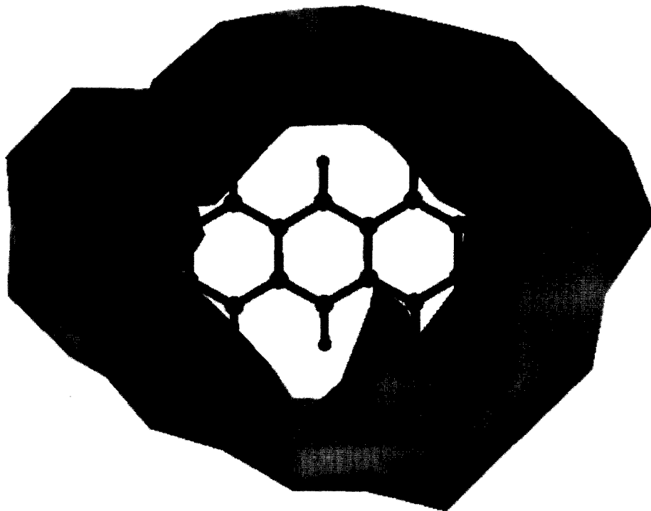
Fig. 3. Plot of the composite CoMFA STDEV*COEFF steric contour for the entire training set of PAHs. Anthracene, a representative PAH, is shown placed in its properly aligned position inside the field. The contours depict regions where increased steric bulk contributes to a larger \Delta_{\text{sub}}H_m^0 (298.15 K) value. The x-axis coincides with the long molecular axis, while the y-axis is normal to the x-axis and in the molecular plane.
