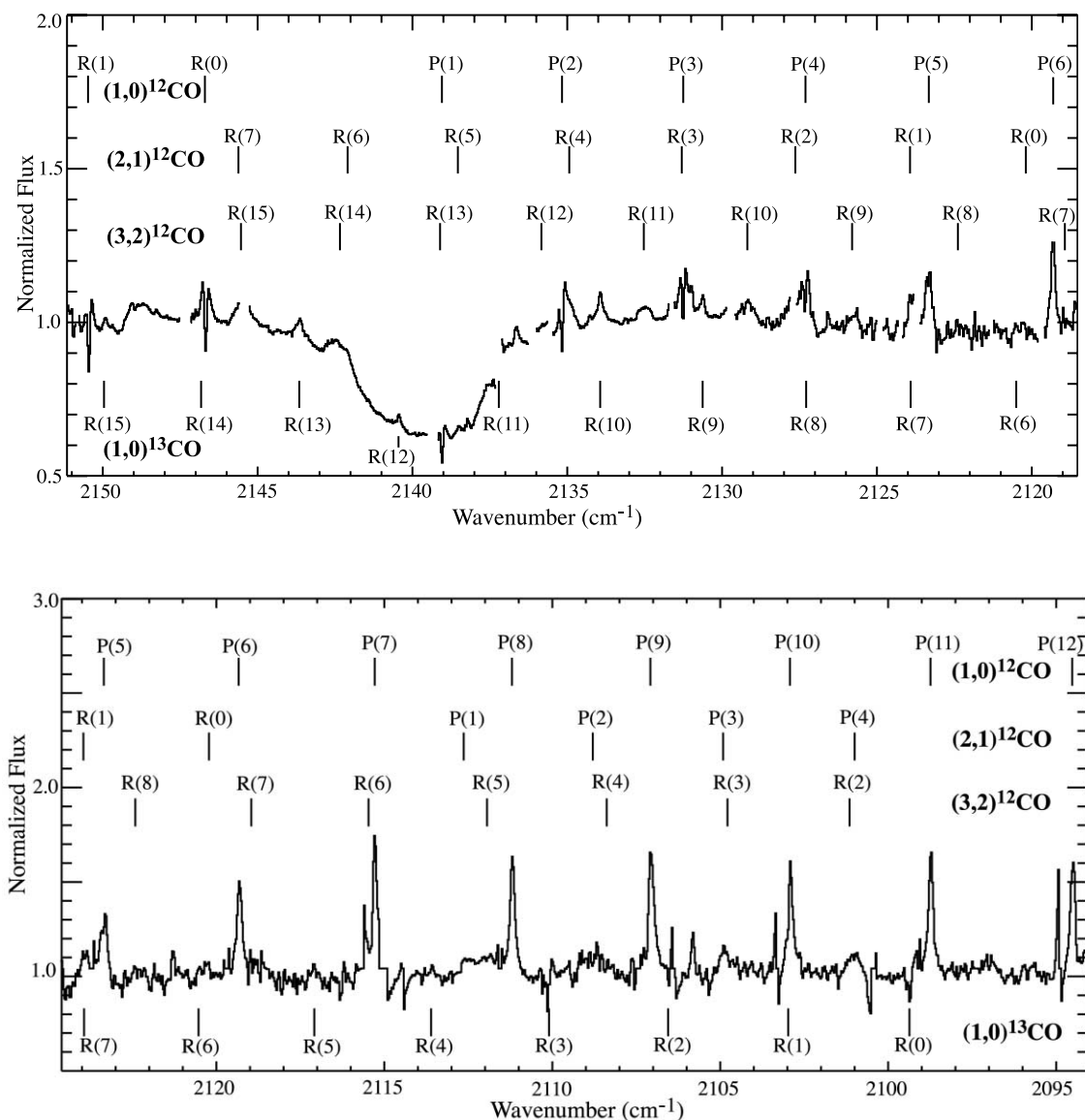
FIG. 1.—Sample spectra showing CO emission features for 12 CO (1–0), (2–1), and (3–2) and 13 CO. In the top panel the broad absorption feature at 2140 cm -1 is due to CO ice. The 12 CO emission lines have narrow absorption components superposed on the low- J lines only out to P(4) . The higher transitions of CO are detected to about P(44) ; none of the high- J lines show signs of CO absorption. The atomic hydrogen line Pf\beta was not detected at 2149 cm -1 (e.g., Simon et al. 2004). Our observations do not cover the Br\alpha at 4.05 \mu m or the Br\gamma line at 2.17 \mu m.
