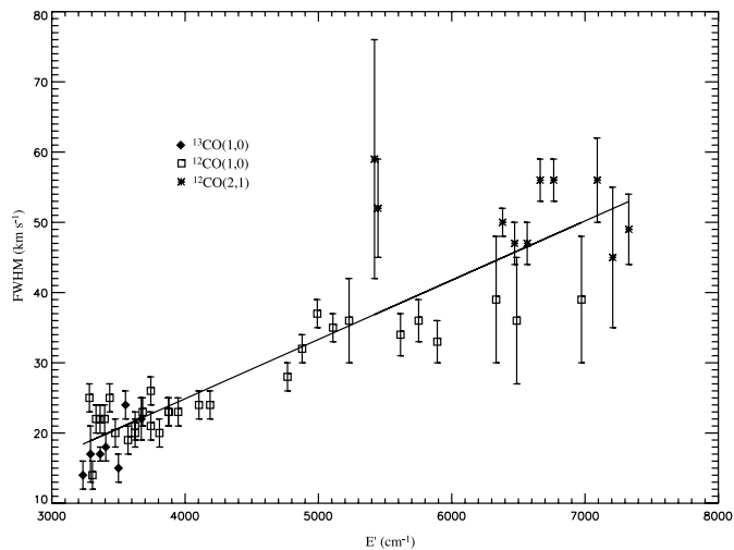
FIG. 3.—Width of the CO emission lines as a function of CO energy level. The open squares denote ^{12}\text{CO} (1, 0). The diamonds indicate ^{13}\text{CO} transitions, which are only detected for the low- J lines. The asterisks represent ^{12}\text{CO} (2, 1) lines, which are only detected for the high- J lines and probably originate nearest the star. The line widths increase with energy (and thus J -value), suggesting that the hotter material observed in the higher J lines is rotating faster, nearer the central star.
