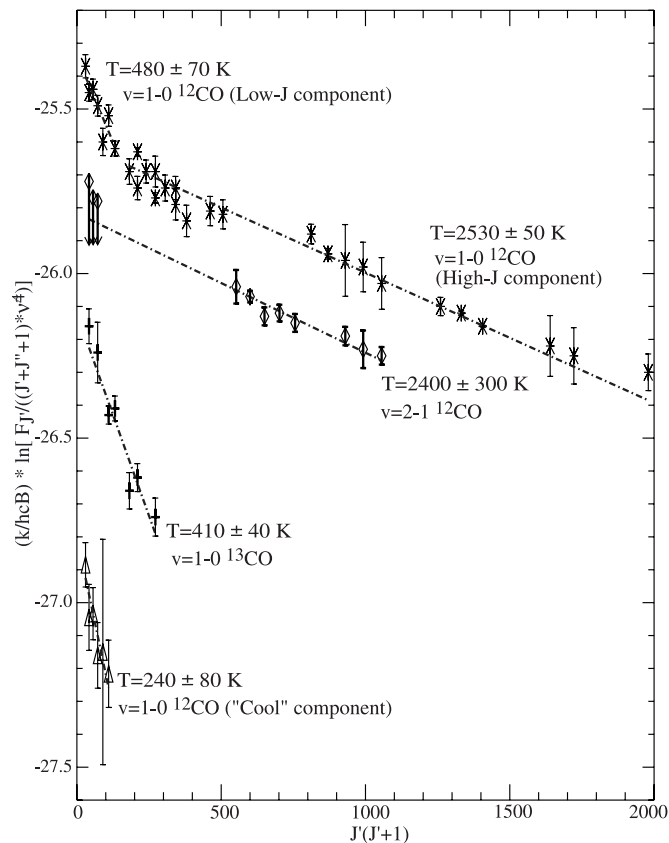
FIG. 2.—Rotational diagram of the CO emission lines for ^{12}\text{CO} (1–0) (hot and cold gas), ^{12}\text{CO} (2–1), and ^{13}\text{CO} (1–0). At the bottom of the figure, a corrected plot for the cooler ^{12}\text{CO} (1–0) gas is presented. A plot of (k/hcB) \ln\{F_{J''}/[\tilde{\nu}^4(J'+J''+1)]\} vs. J'(J'+1) reveals a straight line for optically thin LTE gas, such that the negative reciprocal of the slope is the rotational temperature of the gas. The fit to the ^{12}\text{CO} (1–0) and ( v=2-1 ) high- J lines is linear and provides rotational temperatures of 2530 \pm 50 and 2400 \pm 300 K, respectively. The ^{13}\text{CO} (1–0) provides a rotational temperature of 410 \pm 40 K. The linear fit to the low- J ^{12}\text{CO} (1–0) lines, with the flux contribution from the high- J lines removed, is presented at the bottom. These lines show the largest uncertainty after the warm CO component is subtracted.
