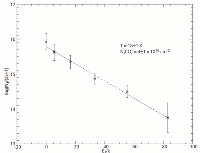
FIG. 4.—Rotational temperature diagram of the cold ^{12}\text{CO} (1-0) absorption component. The linear fit to the plot (using b = 0.85 ) indicates that the optical depth effects have been corrected. The inverse slope of the plot is proportional to the rotational temperature ( 18 \pm 1 \text{ K} ).
