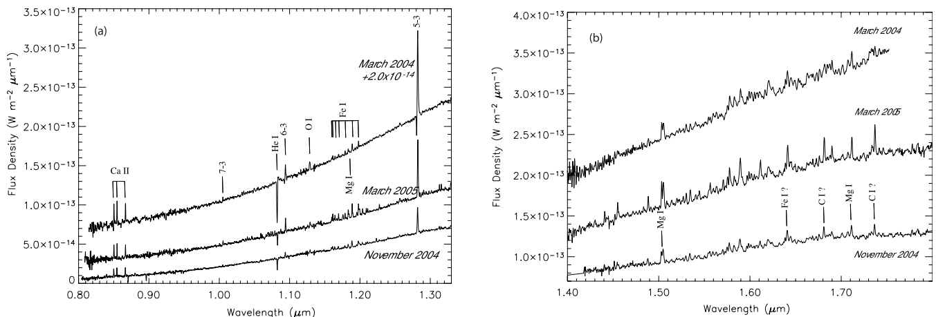
FIG. 1.—SpeX SXD spectra in 2004 March (during outburst) and November and 2005 March (postoutburst) illustrate the similarities and differences with time. (a) The wavelength region from 0.8 – 1.3 \mu\text{m} . (b) The 1.4 – 1.8 \mu\text{m} wavelength region. The 2004 March data in (a) were shifted vertically ( +2 \times 10^{-14} ) to separate the spectra.
