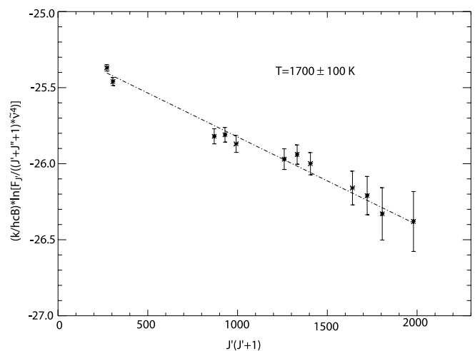
FIG. 4.—Excitation diagram of the 12 CO (1–0) emission lines observed on 2004 July 31. The fit to the high- J lines is linear and gives a rotation temperature of 1700 \pm 100 K, somewhat lower than the \sim 2500 K derived from 2004 February observations.
