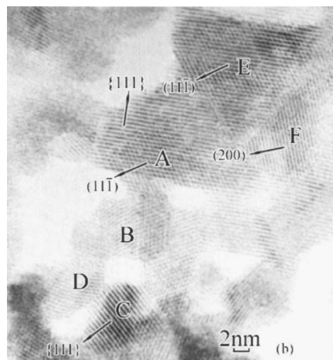
FIG. 9. HRTEM images of the six WC_{1-x} nanocrystals in Fig. 8, after a single tilt of 14.5^\circ around the side-entry goniometer tilt axis.
