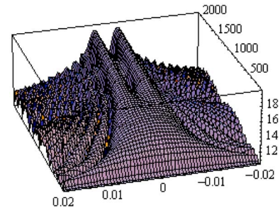
FIG. 15. (Color online) Logarithmic fringe-intensity profile ( d=2 \text{ \AA} and \lambda=0.01 \text{ \AA} ) for a spherical particle whose diameter t is given in angstroms by the top-labeled axis (running front to back), as a function of “tilt from edge-on in radians” on the bottom-labeled axis (running left to right).
