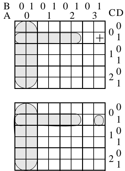
Figure 2. A visualization of the “new event” operator.
